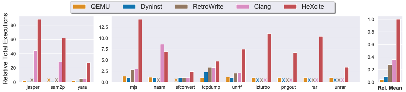
Figure 9: HeXCITE’s mean throughput relative to conventional coverage tracers. We normalize throughput to the worst-performing tracer per benchmark, and compute each tracer’s mean performance relative to HeXCITE’s across all benchmarks (shown in the rightmost plot). For each benchmark we omit incompatible tracers (denoted by a colored X). All comparisons to HeXCITE yield a statistically significant difference (i.e., Mann-Whitney U test p < 0.05 ).
